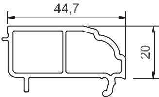
Remate monorriel 7405
